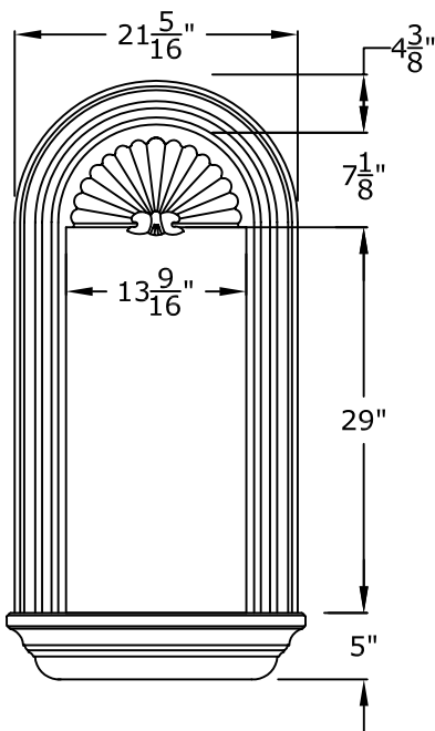
Clamshell
